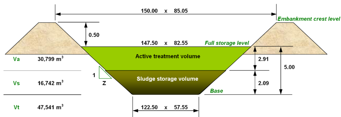
Figure 2. An example of the schematic drawing of the primary anaerobic pond provided on the 'Anaerobic pond design' sheet of PigBal 4.
